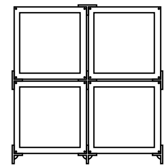
BUNKE (4x element + 4x connection cross + 10x connection side)
